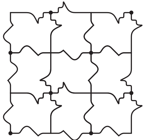
TesCFf & TesCFfs TesCFf1 & TesCFf1s (checkerboard)
